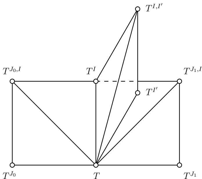
FIGURE 7. The star of T in K . The star of T in W is the “V” subcomplex spanned by T^{J_0, I} , T , T^{J_1, I} .
