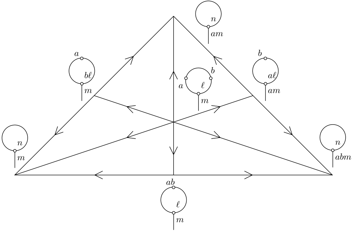
FIGURE 13. The 2-cell in W_{p,q} in Lemma 3.4. The labels 1 and p are omitted from the figure.
