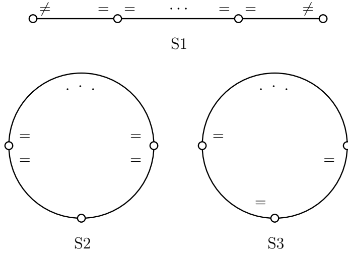
FIGURE 1. Shelters in T/G . The “=” signs denote when an inclusion G_e \subseteq G_v is an equality. The “ \neq ” signs denote when an inclusion is proper. Other inclusions may or may not be proper.
