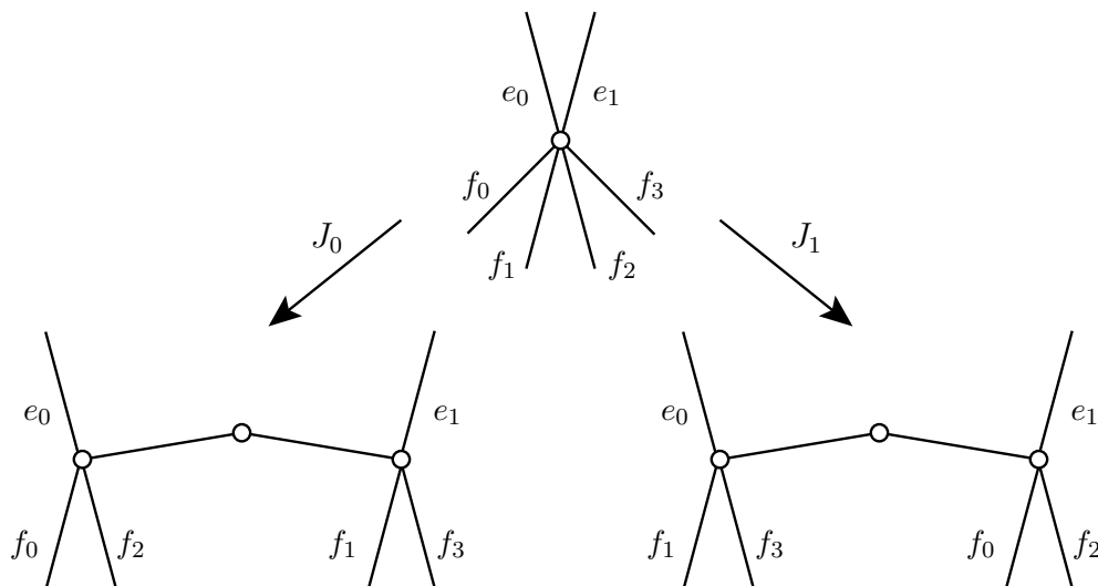
FIGURE 6. The expansions defined by J_0 and J_1 .
