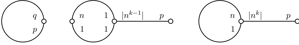
FIGURE 11. Labeled graphs representing G_{p,q} -trees in W_{p,q} when |n| is prime ( k \geq 1 ).
