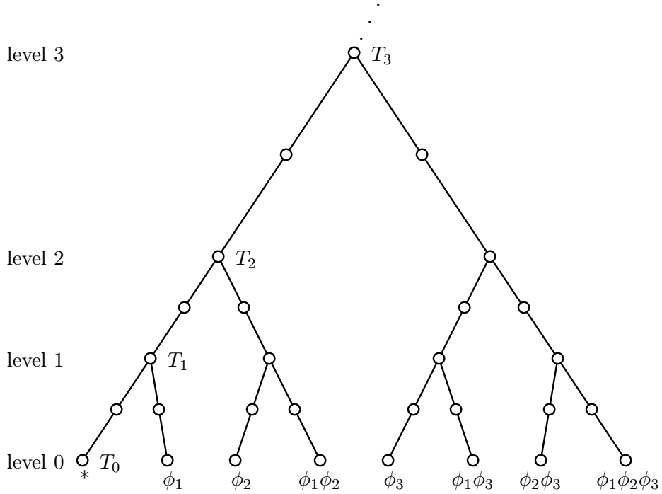
FIGURE 12. A piece of the complex W_{2,4} . The labels on the bottom show the action of the automorphisms \phi_k listed in (4).
