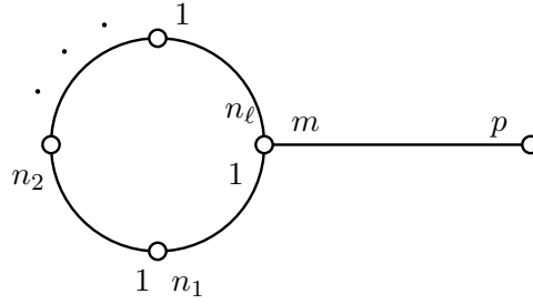
FIGURE 10. Labeled graphs representing G_{p,q} -trees in W_{p,q} . The labels on the circuit \gamma satisfy n_1 \cdots n_\ell = n and |n_s| \neq 1 with the possible exception of n_\ell .
