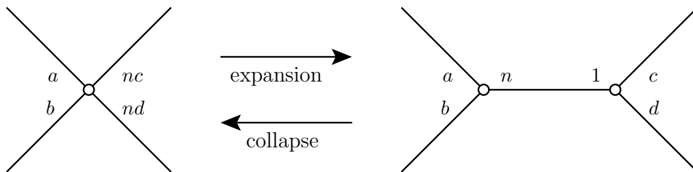
FIGURE 3. The effect of elementary moves on labeled graphs.
