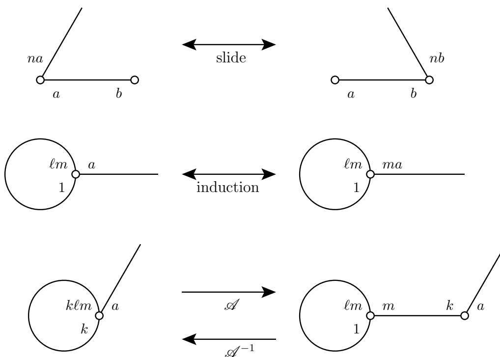
FIGURE 4. The effect of the special elementary deformations described in Section 1.1 on labeled graphs. These three moves suffice to relate any two reduced labeled graphs representing the same GBS group.
