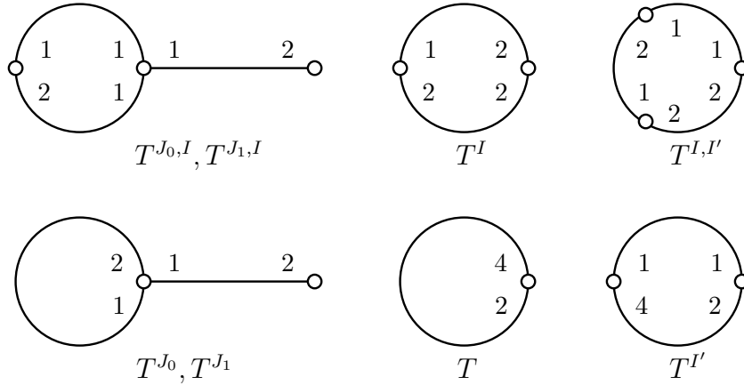
FIGURE 5. The labeled graphs for BS(2, 4) representing the vertices in the star of T in K .
