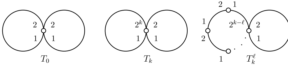
FIGURE 8. Labeled graphs representing the GBS group in Example 2.2. The deformation retract W for the canonical deformation space for this group is not finite dimensional.
