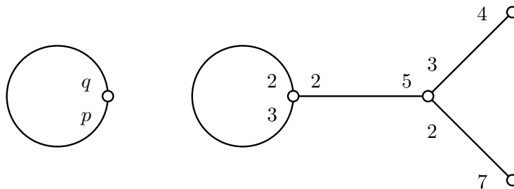
FIGURE 2. Examples of labeled graphs. The labeled graph on the left represents the classical Baumslag-Solitar group BS(p, q) .
