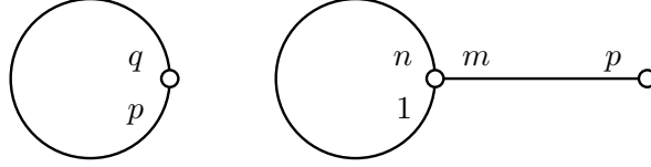
FIGURE 9. Labeled graphs representing reduced G_{p,q} -trees in W_{p,q} , m \in \Pi^+(n) , m \neq 1 .
